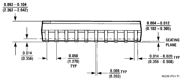
Small Outline (SO) Package Order Number LM1036M or LM1036MX NS Package Number M20B
